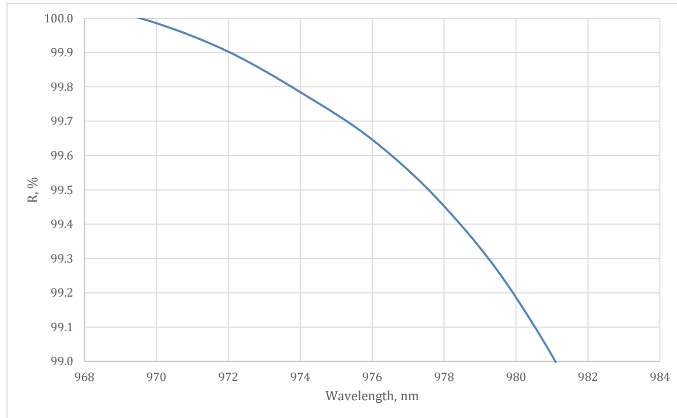
Fig. 1. Measured p-polarization reflectance graph at AOI=45°
