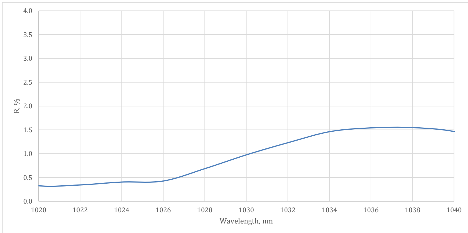
Fig. 2. Measured p-polarization reflectance graph at AOI=45°
