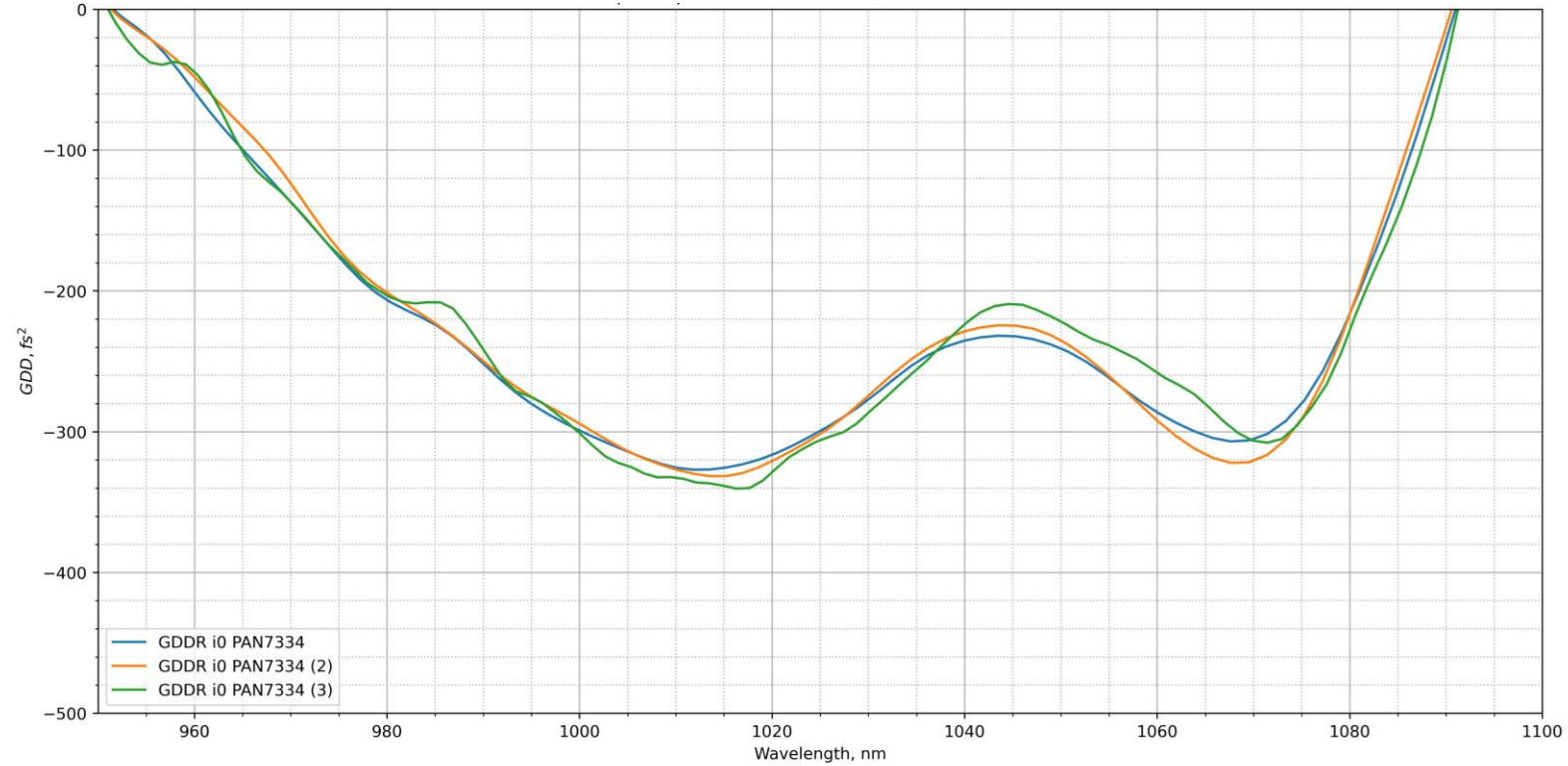
Fig. 2. Measured GDD
