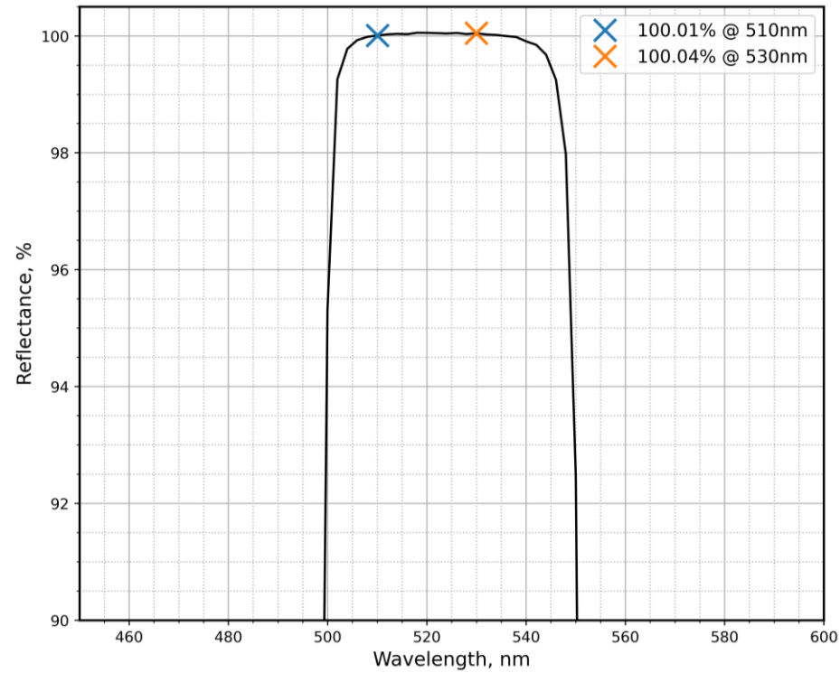
PO5816 Rs i45 grinded test piece S2
