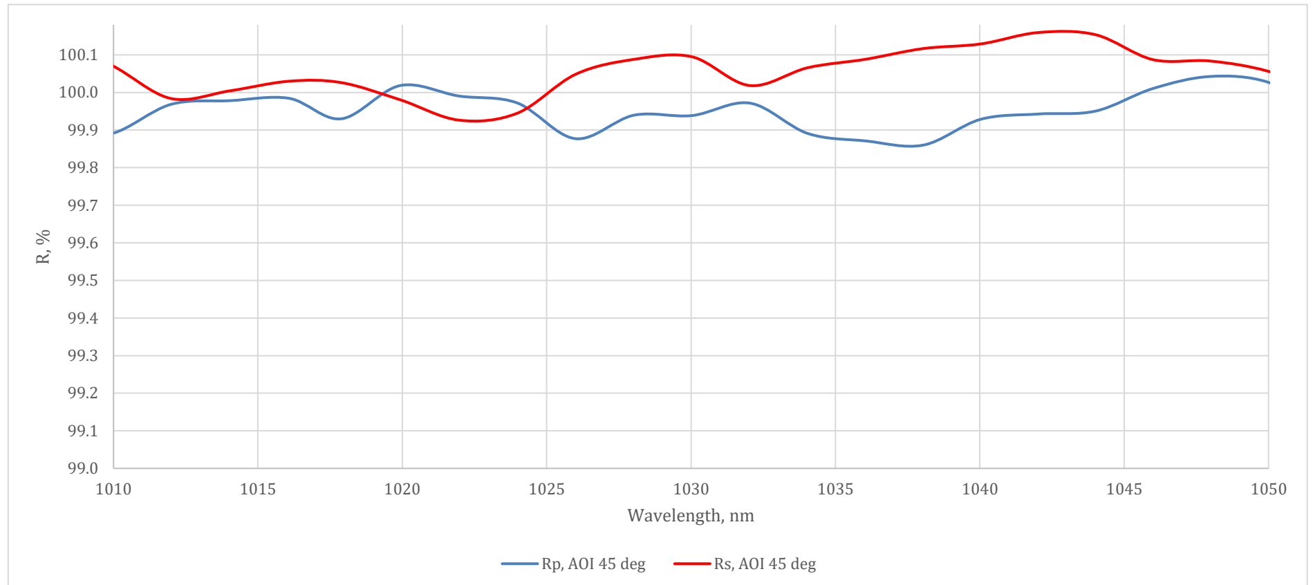
Fig. 1. Measured s and p polarization reflectance graphs at AOI=45°. R over 100% due to measurement errors.
