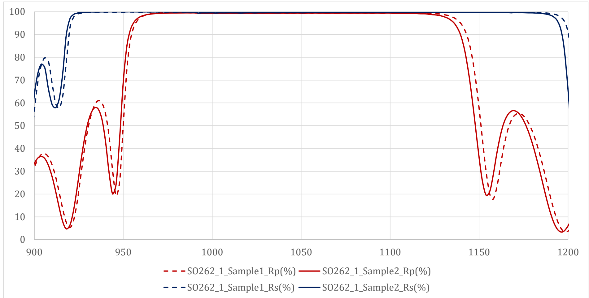
Fig. 1. Measured reflectance graph for s and p polarization components at AOI=45 deg.
